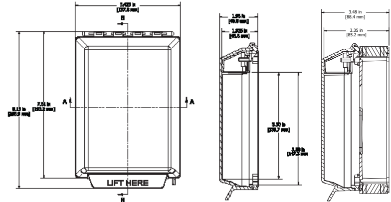
PRODUCT DIMENSIONS
